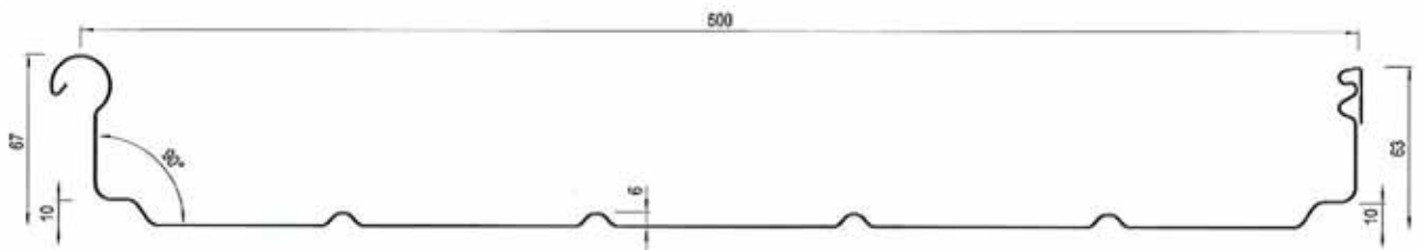
RIB-ROOF Evolution cover width = 500 mm
