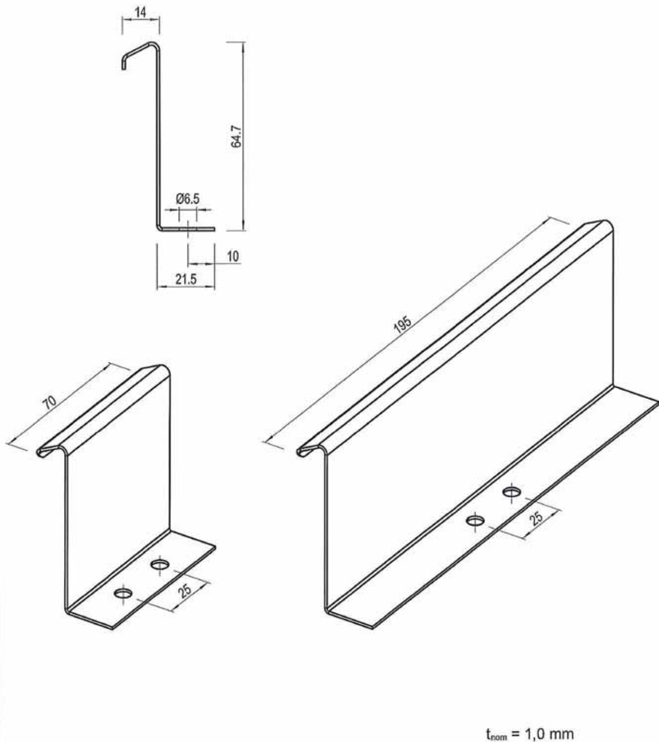
RIB-ROOF Evolution sliding standing seam system aluminium
