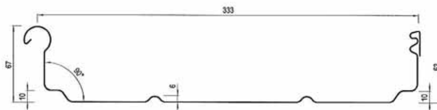
RIB-ROOF Evolution cover width = 333 mm
