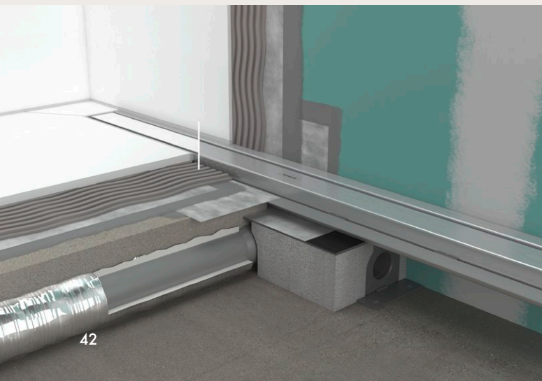
RainDrain Allround standard installation
