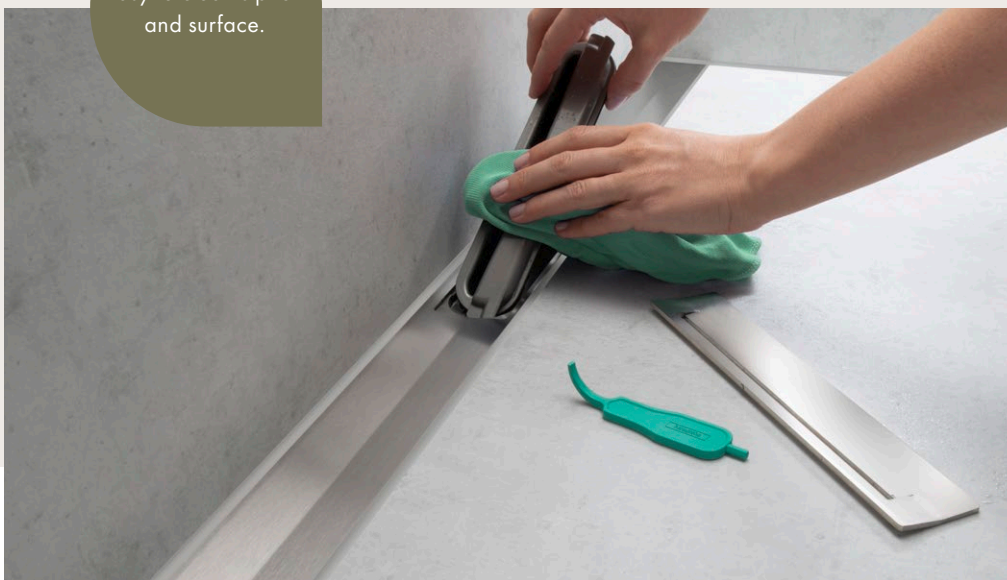
Height adjustment
