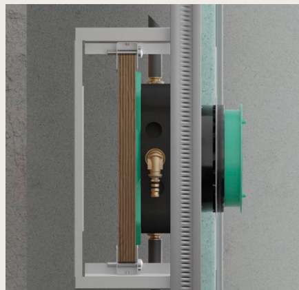
Installation on a carrier system
