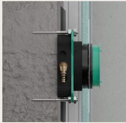
Installation on the wall
