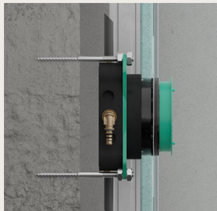
Installation in front of the wall (here using variable spacers with M 10 hanger bolts)
