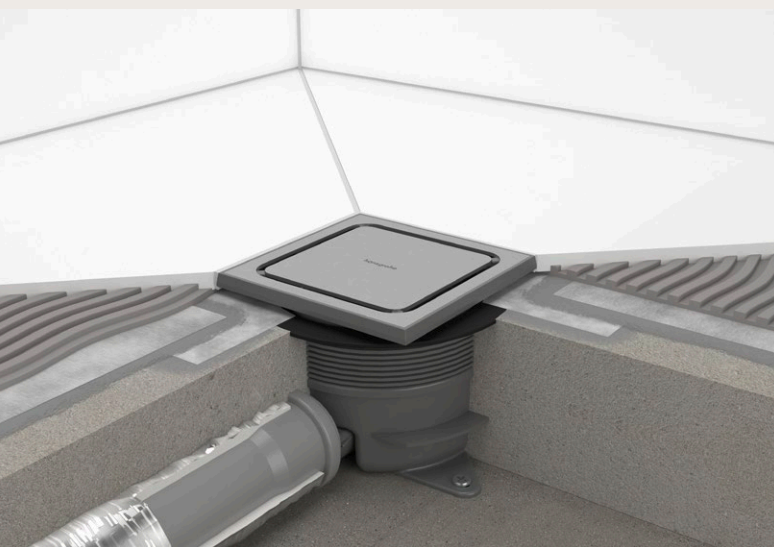
RainDrain Spot Plus with tileable grate
