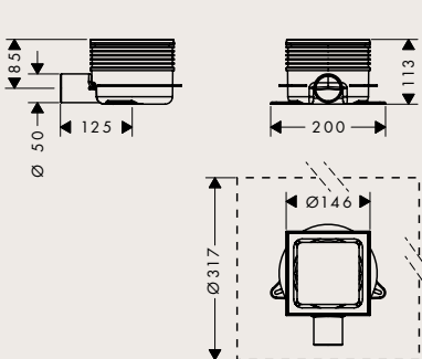
RainDrain Spot Plus
