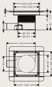
RainDrain Brilliance 150 mm
