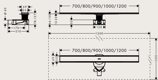
RainDrain Allround flat installation
