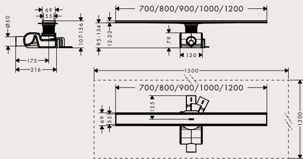
RainDrain Allround standard installation
