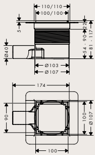
RainDrain Brilliance 100 mm
