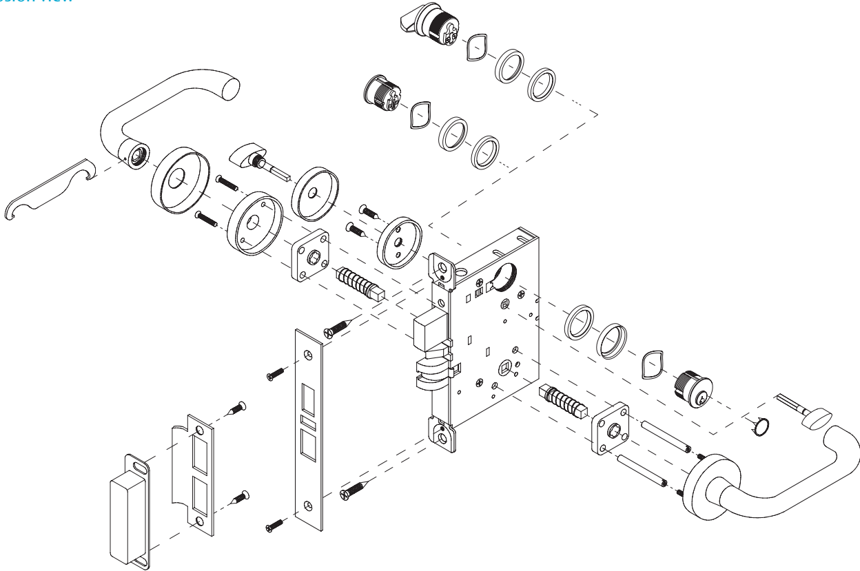
Explosion view
